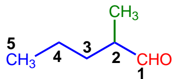
2-methyl-pentanal
