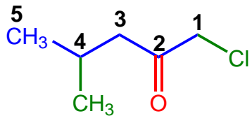
1-chloro-4-methyl-pentan-2-one
